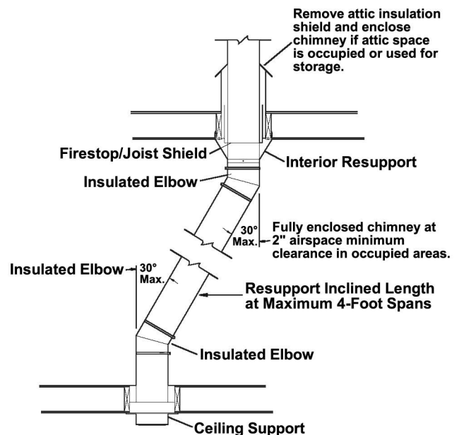
Figure 4 Elbow Installation
