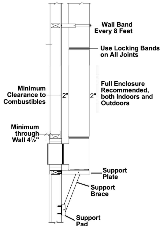
Figure 1 Wall Support for 10"
