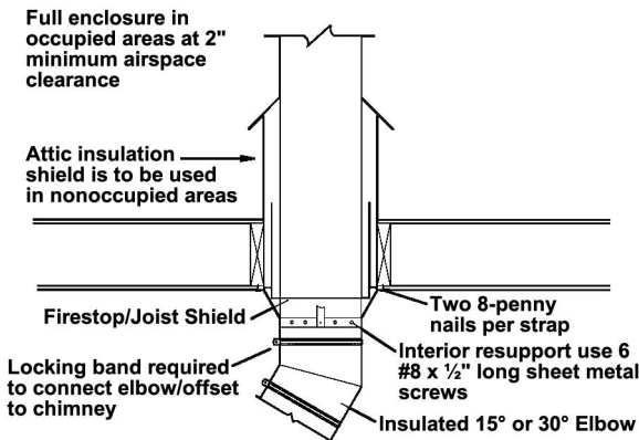
Figure 5 Interior Resupport Use when the installation of an interior resupport below a locking band is not possible.
